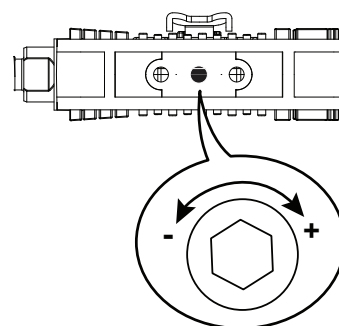
Disengage (release)
