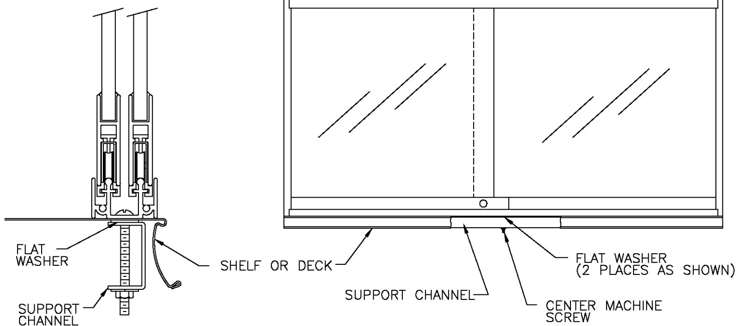
FIGURE IIA END VIEW
