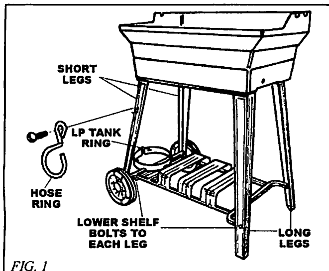
Complete View of Cart Assembly
